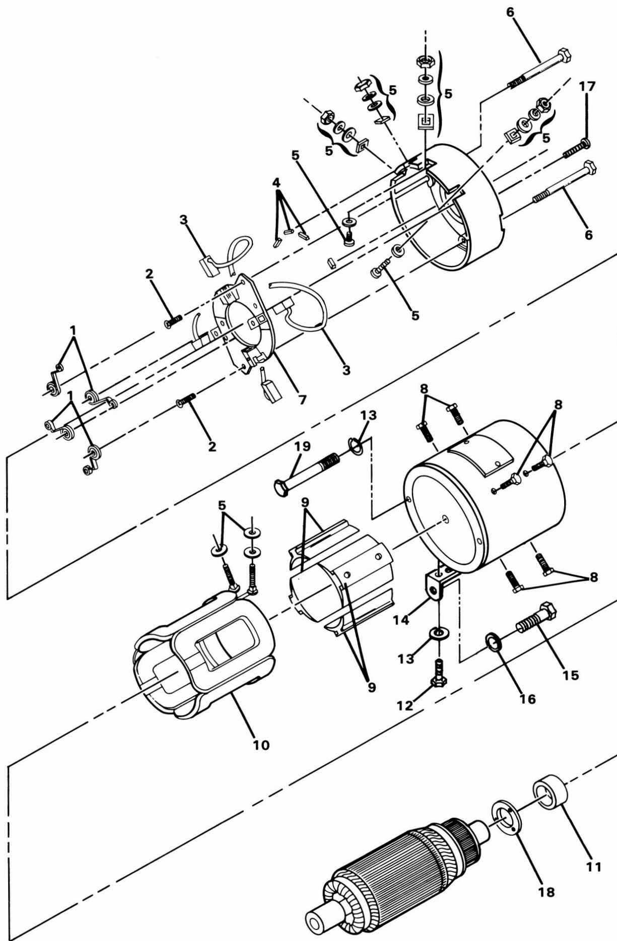
MOTOR ASSEMBLY FOR CLUB CAR MODELS 1012191 AND 1014678
